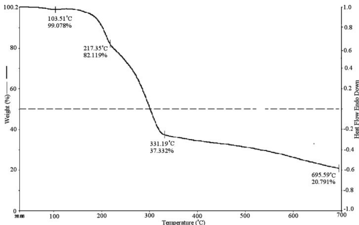
Figure 4. Thermogravimetric analysis of 1b as a function of temperature.
