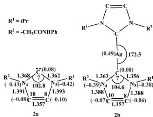
Figure 2. Calculated key structural parameters of free carbene 2a and the complex 2b . NPA charges are given in parentheses.
