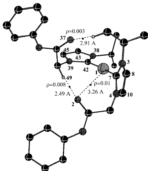
Figure 3. The B3LYP/SDD,6-31G* optimized geometry of 2b showing weak intramolecular interactions and the corresponding densities at the bond critical points ( \rho_{bc} ) computed using the AIM theory (only selected hydrogen atoms are shown for clarity).
