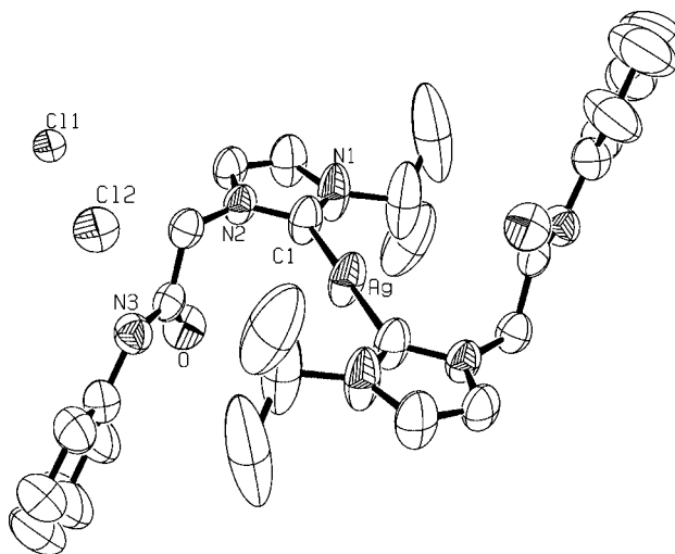
Figure 1. ORTEP of 1b . The \text{Cl}^- ion is disordered with C11 having 1/3 occupancy and C12 having 2/3 occupancy. Selected bond lengths [Å] and angles [°]: Ag–C(1) 2.085(3), N(1)–C(1) 1.350(4), N(1)–C(2) 1.379(4), C(1)–Ag–C(1) 180.000(1), N(2)–C(1)–N(1) 104.0(2), N(2)–C(1)–Ag 124.7(2), N(1)–C(1)–Ag 131.3(2).
